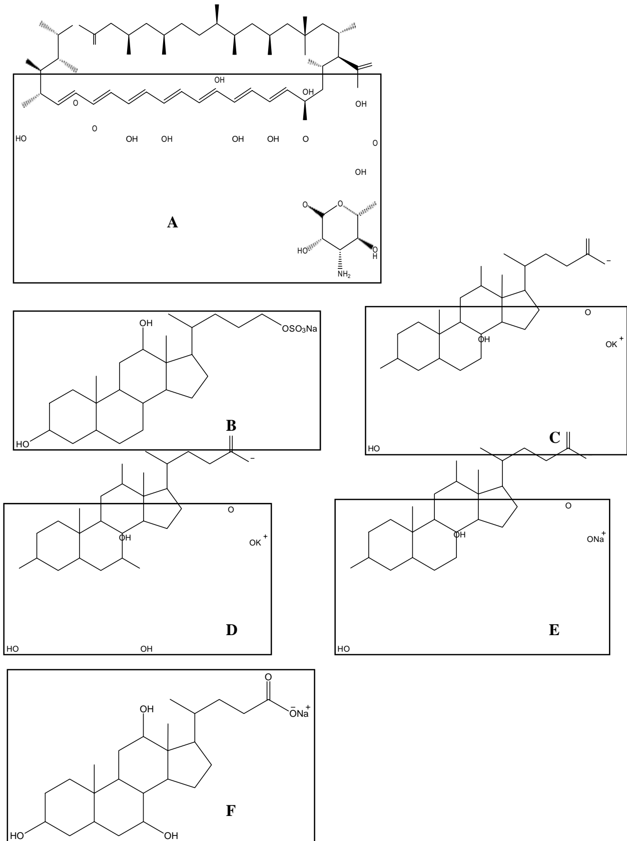
Figure1. The chemical structure of Amphotericin B (A), Sodium deoxycholate sulfate (B), Potassium deoxycholate (C), Potassium cholate (D), Sodium deoxycholate (E) and Sodium cholate (F).
