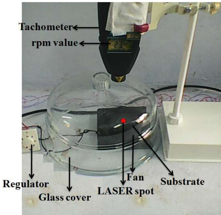
Figure 1. Lab Made Spin Coater
