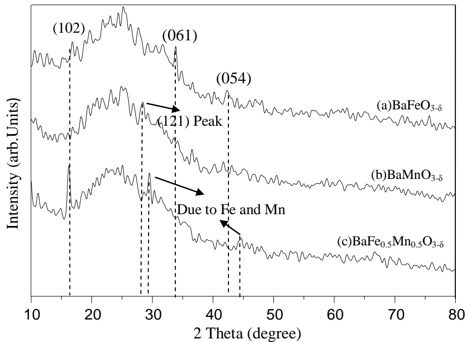
Figure 3. XRD pattern of \text{BaFe}_x\text{Mn}_{1-x}\text{O}_{3-\delta} films ( x=0, 0.5, 1 )
