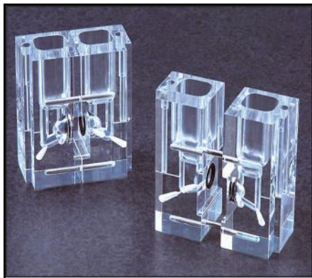
Fig. 7 Picture of Ussing chamber
